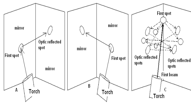
Fig. 2A, B, C: Physical optical reflection phenomenon was observed sending a laser light of a torch towards the area between the mirrors (2C) and toward one of the mirrors (2A and 2B) obtaining, respectively, a multiplication and duplication spots. The beam of light was sent by the research before performing the experiments with subjects.
