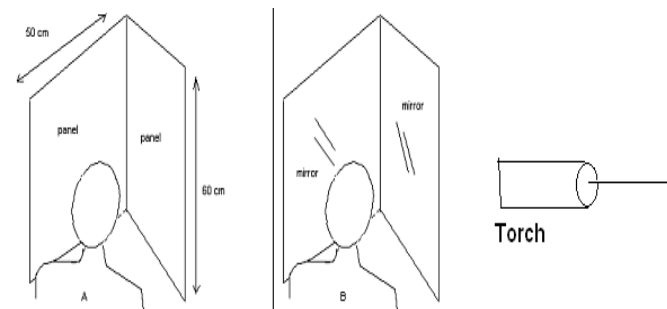
Fig. 1A not reflective cardboard panels Fig. 1B reflective mirrors (see text) 1C Torch (see text)
