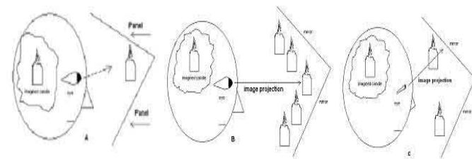
Fig 3 Visual imagery observed after sending mental image toward white no reflecting panels (A) and after sending toward mirrors (B, C). In B and C a physical reflecting like phenomenon appeared.
